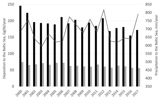
Fig. 9. Time series of wet (black) and dry (grey) depositions to the Baltic Sea basin during the period 2000–2017. Unit: \text{Gg(N)}\text{ yr}^{-1} , left vertical axis. The grey curve depicts the annual precipitation averaged over the Baltic Sea basin in each year of the trend period. Unit: \text{mm yr}^{-1} , right vertical axis.
