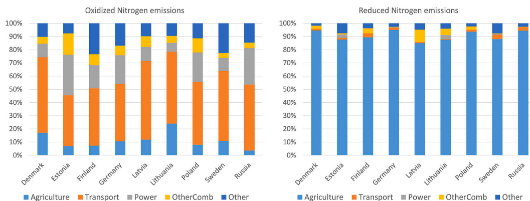
Fig. 3. Percentage contribution from different sectors to each HELCOM country's emission of oxidized and reduced nitrogen in 2017. The sectors are based on the GNFR System (Gridded Nomenclature For Reporting) used by EMEP since 2017. More information about the GNFR sectors, and which processes they include, can be found on the web pages of the EMEP Centre CEIP ( https://www.ceip.at/reporting-instructions , see e.g. Annex 1 to the 2014 Guidelines for Estimating and Reporting Emission Data). Legend of the figure: Agriculture = emissions from livestock and other processes (GNFR Sectors K + L); Transport = aviation (landing/take-off), road traffic, off-road traffic, and inland shipping (GNFR Sectors F + G + H + I); Power = public power generation (GNFR Sector A); OtherComb = other stationary combustion (GNFR Sector C); Other: all other sources (GNFR Sectors B + D + E + J + M).
