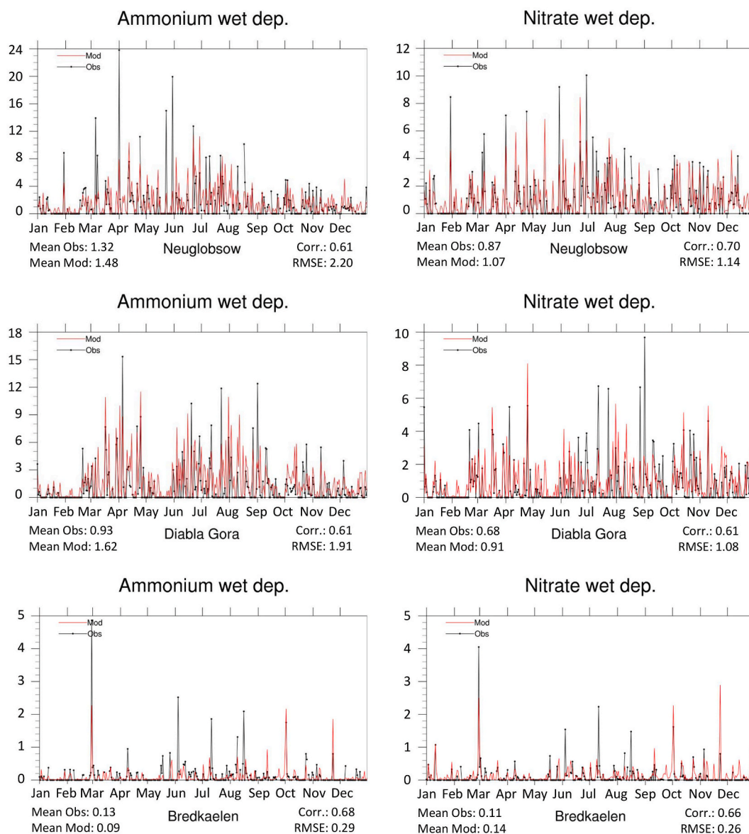
Fig. 2. Model evaluation of the EMEP model for time series of daily modelled and observed wet deposition of nitrogen for the year 2017 at HELCOM measurement stations in Germany (Neuglobsow 53°10'N/013°02'E), Poland (Diabla Gora 54°09'N/022°04'E) and Sweden (Bredkaelen 63°51'N/015°20'E). Unit: \text{mg(N)} \text{ m}^{-2} \text{ day}^{-1} . Large peaks are usually related to heavy-precipitation events.
