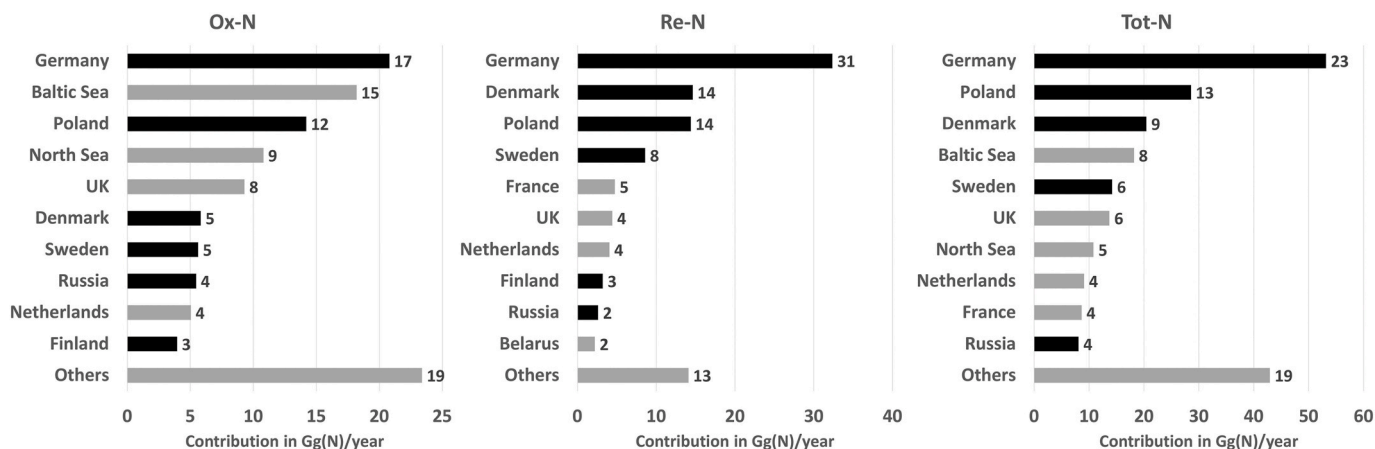
Fig. 11. Contributions from the top-10 sources contributing to the actual (not weather-normalized) deposition of oxidized, reduced and total (oxidized + reduced) nitrogen deposition to the Baltic Sea in 2017. Unit: Gg(N) yr -1 . The labels behind each bar give the fractional contribution to the total (in %).
