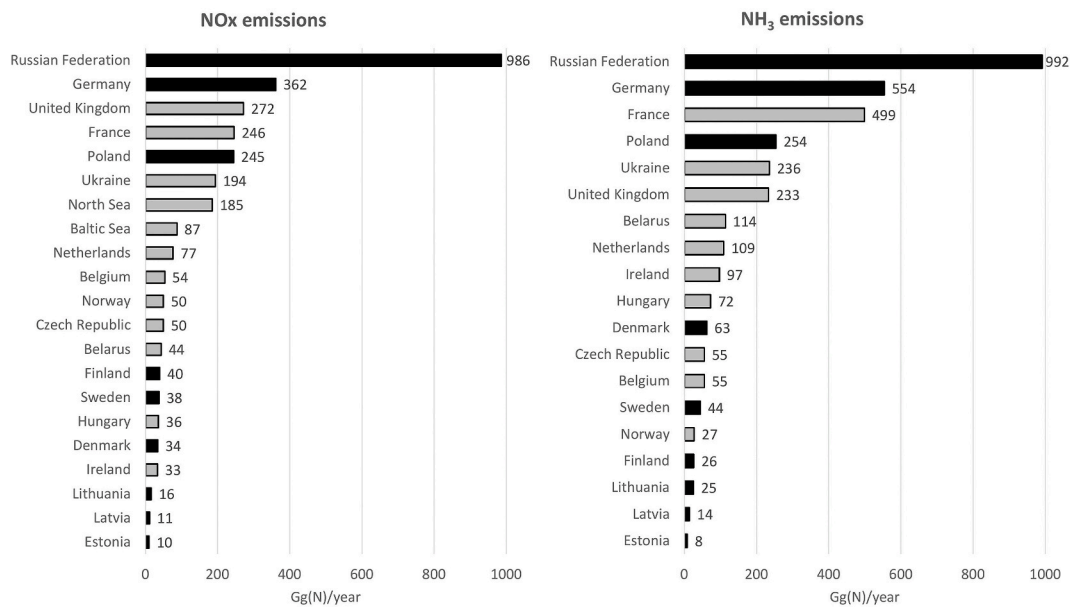
Fig. 5. Ranked list of emitters of nitrogen oxides and ammonia in 2017. Only emission sources contributing more than 1% to nitrogen deposition to the Baltic Sea basin are shown. Emissions from HELCOM Contracting Parties are marked in black. The numbers given here for Russia, which is not fully covered by the EMEP model domain, include only emissions within the domain (outlined in red in Fig. 1). ‘North Sea’ and ‘Baltic Sea’ represent emissions from shipping in these sea areas. Unit: Gg(N) yr -1 .
