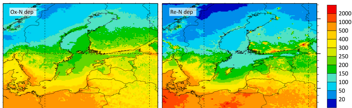
Fig. 7. Depositions of nitrogen oxides (left) and ammonia (right) in the year 2017, as calculated by the EMEP model for the Baltic Sea and its surroundings. Grid resolution: 0.1°×0.1°. Unit: mg(N) m -2 yr -1 .
