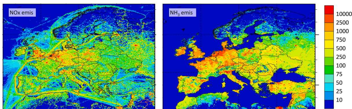
Fig. 4. Emissions of nitrogen oxides (NO x ) and ammonia (NH 3 ) in the year 2017 as provided by CEIP for use in the EMEP model. The grid resolution is 0.1^\circ \times 0.1^\circ . Unit: \text{mg(N) m}^{-2} \text{yr}^{-1} .
