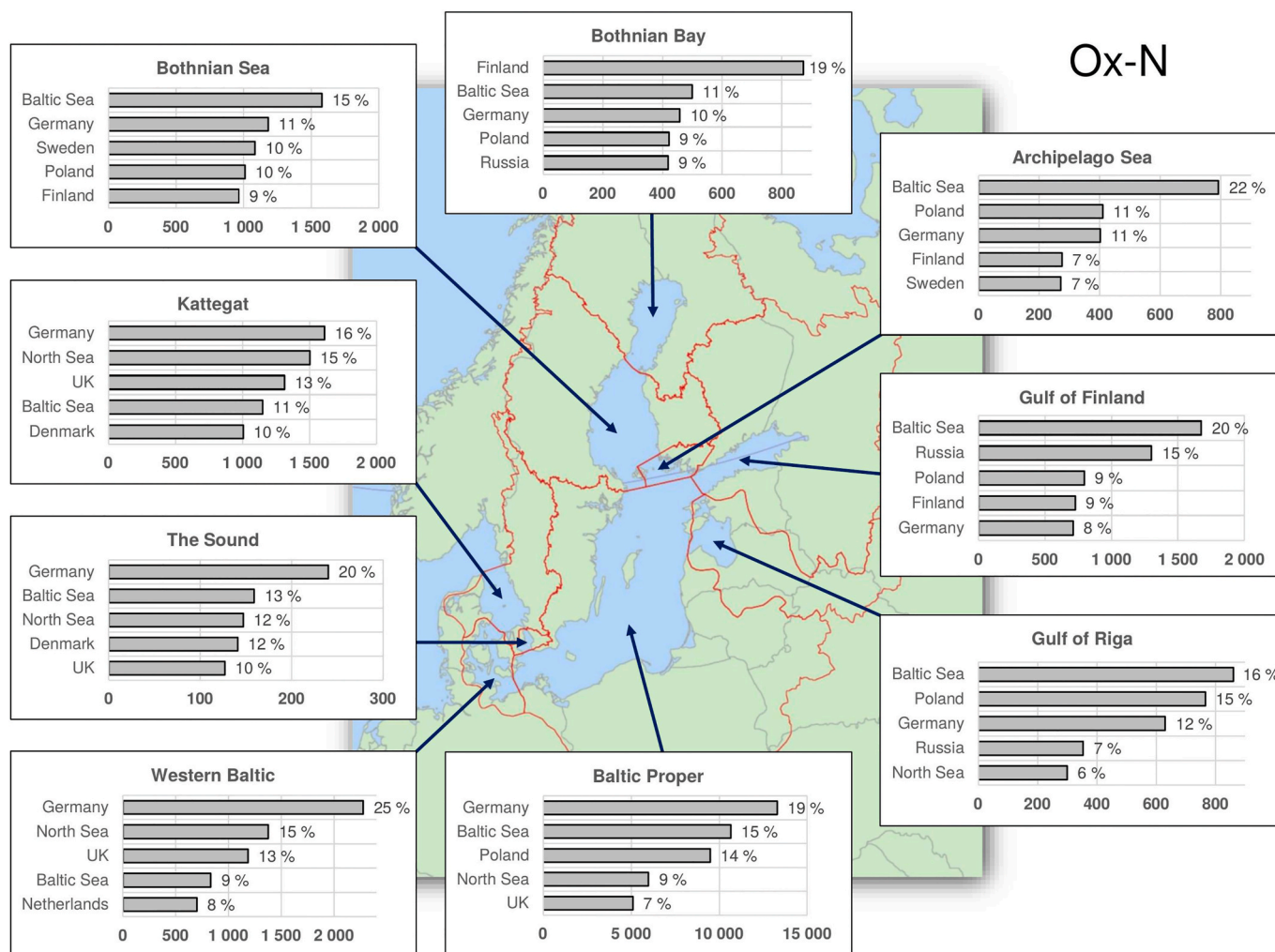
Fig. 12. Contributions of top-5 contributing countries to oxidized nitrogen deposition to the Baltic Sea sub-basins in the year 2017. Unit: Mg(N) yr -1 . The labels at each bar indicate the country's percentage of the total deposition of oxidized nitrogen to the respective sub-basin.
