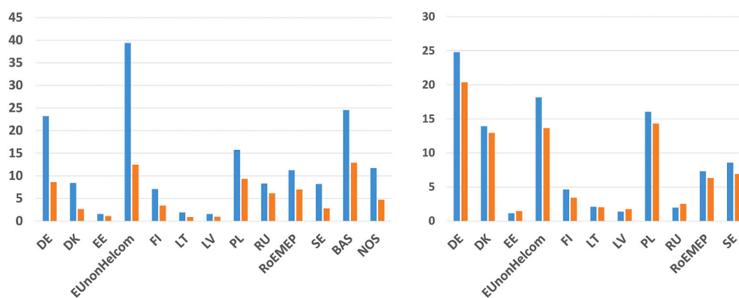
Fig. 15. Contributions from different sources to nitrogen deposition in 2005 (blue bars) and in 2030 (red bars). Left: Oxidized nitrogen, right: reduced nitrogen. Unit: \text{Gg(N) yr}^{-1} . For definitions of BAS, NOS, EUnonHelcom, and RoEMEP see caption of Table 3. (For interpretation of the references to colour in this figure legend, the reader is referred to the Web version of this article.)
