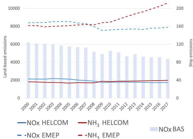
Fig. 6. Annual emissions of nitrogen oxides (blue) and ammonia (red) from all EMEP sources (dashed lines, left vertical axis), from HELCOM sources (solid lines, left vertical axis) and from the ship emissions on the Baltic Sea (bars, right vertical axis) in the period 2000–2017, based on emission data provided by CEIP for modelling. Note that ships emit nitrogen only in the form of NOx (not ammonia). Unit: Gg(N) yr -1 . (For interpretation of the references to colour in this figure legend, the reader is referred to the Web version of this article.)
