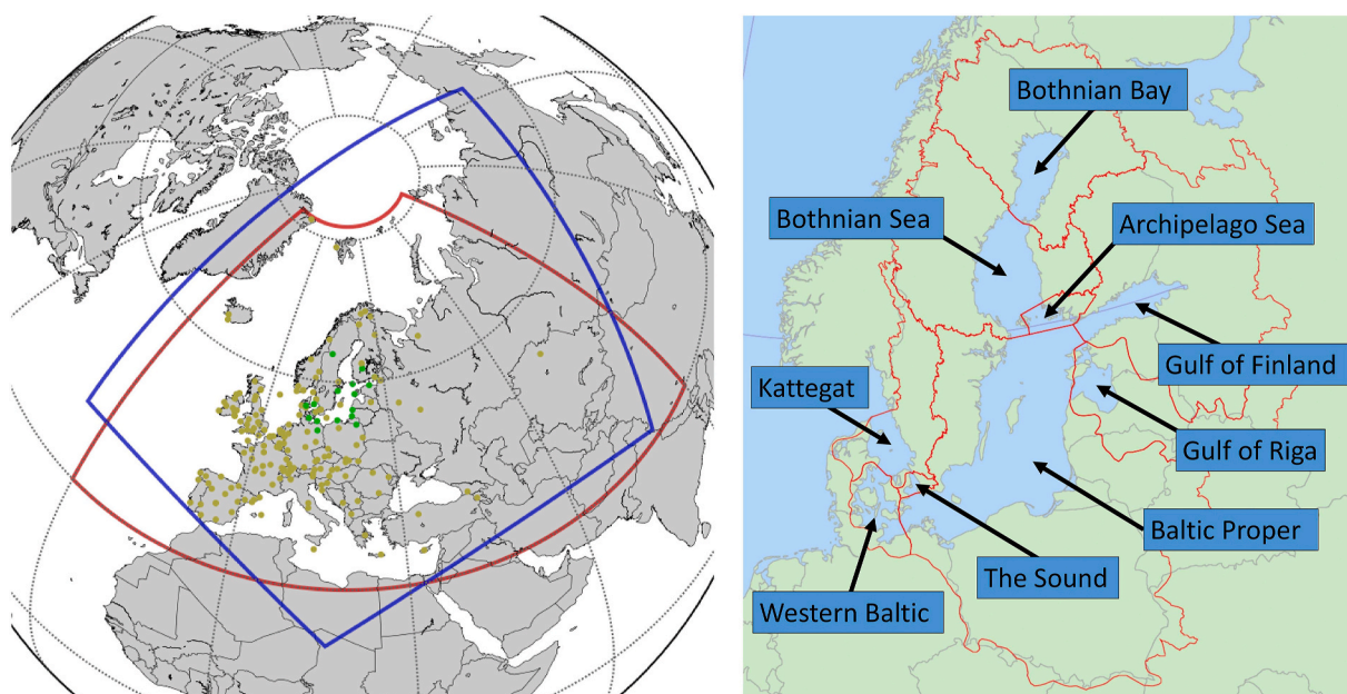
Fig. 1. Left: EMEP model domains. Red outline: Longitude latitude grid covering the geographic area between 30°N and 82°N and 30°W-90°E used for the status and trend studies of Sections 3 and 4; blue outline: polar-stereographic grid used for the source-receptor and future simulations of Sections 4 and 5. Sites measuring nitrogen components are indicated by dots (green: HELCOM sites, yellow: all other sites). Right: The nine sub-basins of the Baltic Sea and their catchment areas. (For interpretation of the references to colour in this figure legend, the reader is referred to the Web version of this article.)
