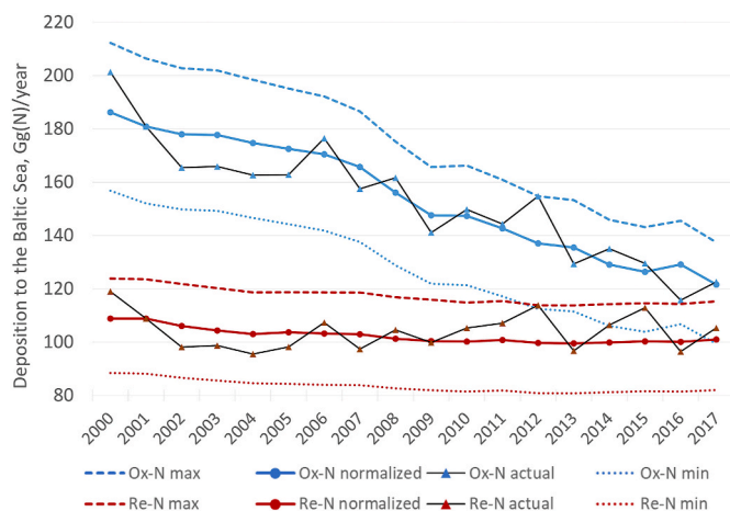
Fig. 8. Time series of depositions of oxidized (blue) and reduced (red) nitrogen to the entire Baltic Sea basin during the period 2000–2017. Unit: \text{Gg(N)}\text{ yr}^{-1} . Actual, normalized, maximum and minimum values are shown (for methods and definitions see Section 2.3). Note that the vertical axis does not start at zero; thus the long-term trends and year-to-year variability may appear larger than they are. (For interpretation of the references to colour in this figure legend, the reader is referred to the Web version of this article.)
