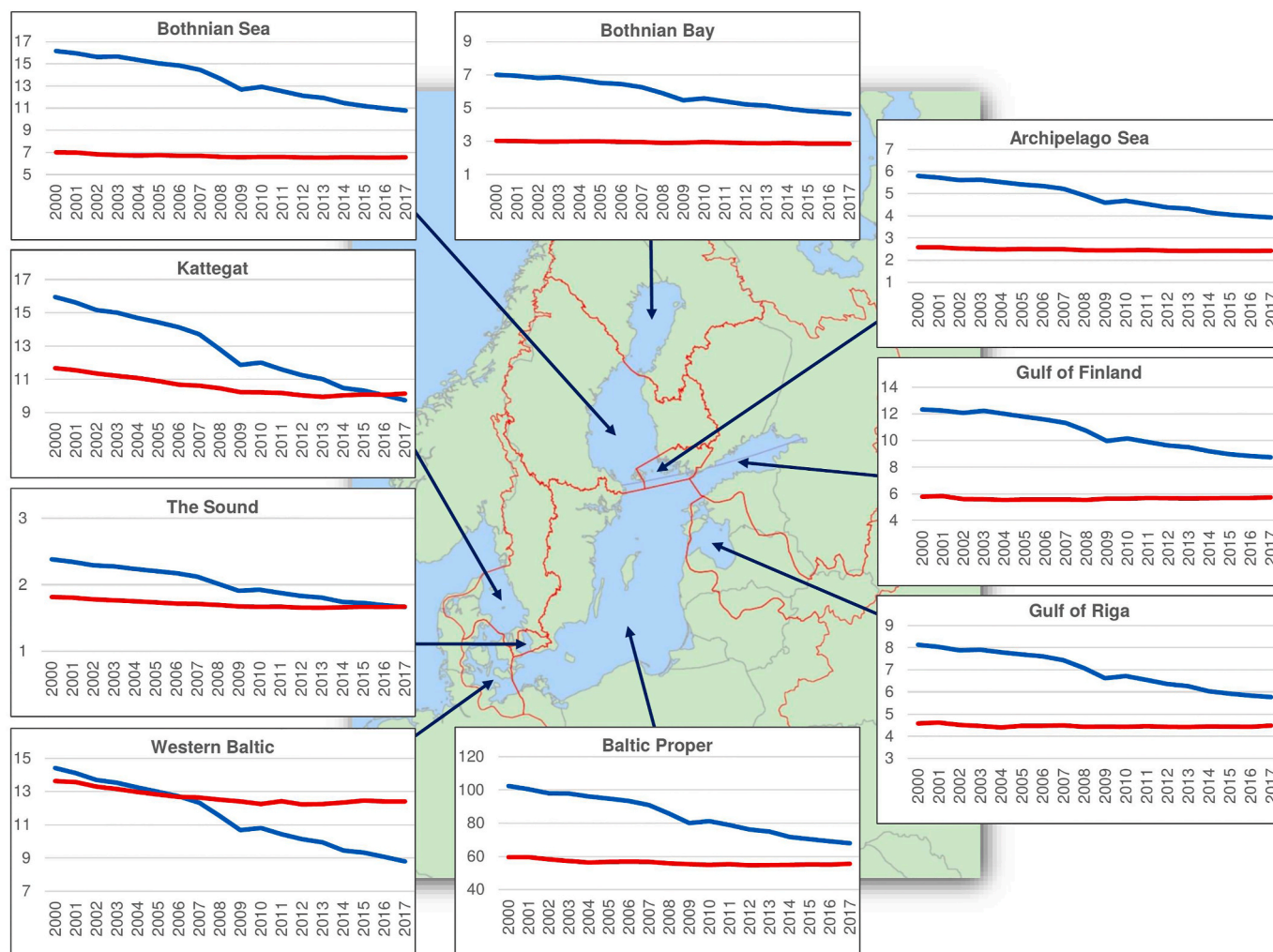
Fig. 10. Time series of normalized depositions of oxidized (blue) and reduced (red) nitrogen to the nine sub-basins of the Baltic Sea in the period 2000–2017. Unit: \text{Gg(N) yr}^{-1} . Note that the vertical axes do not start at zero; trends and year-to-year variability may thus appear larger than they are. (For interpretation of the references to colour in this figure legend, the reader is referred to the Web version of this article.)
