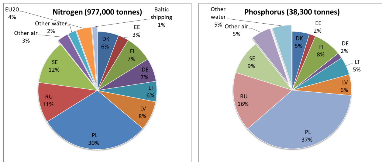
Figures 3.1a and 3.1b. Total actual water- and airborne inputs of nitrogen and phosphorus to the Baltic Sea in 2010 by HELCOM Contracting Parties and other sources. Atmospheric nitrogen deposition is divided into Baltic shipping, EU20 (the 20 non-HELCOM EU countries including Croatia) and 'other air' - which for nitrogen is other non-HELCOM countries and other distant sources (such as North Sea shipping) and for phosphorus all atmospheric sources. 'Other water' is transboundary waterborne inputs from non-HELCOM Contracting Parties entering the Baltic Sea (see Table 3.3a ). See also note to Table 2.2 regarding the pre-conditions on the PLC-5.5 data set.
