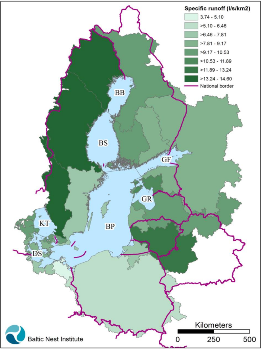
Figure 3.3a. Area-specific run-off (water flow, l s^{-1} km^{-2} ) in 2010 calculated per main sub-catchment and per country. See note to Table 2.2 regarding the pre-conditions on the PLC-5.5 data set.
