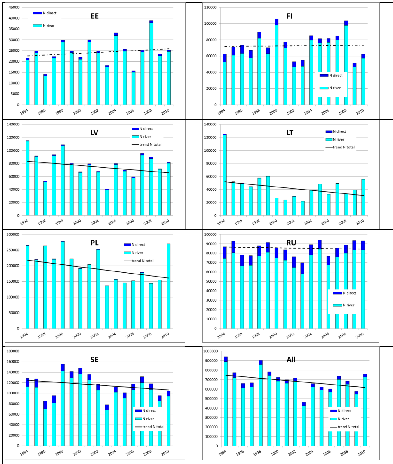
Figure 2.4a. Actual annual total riverine + direct (waterborne) nitrogen inputs by Contracting Party to the Baltic Sea and the total inputs to the Baltic Sea. The trend for the flow normalized waterborne total nitrogen input is inserted as a line to indicate a possible trend (solid line = a statistically significant trend; dotted line = no statistically significant trend; see further explanations in Chapter 2.4 ). See note to Table 2.2 regarding the pre-conditions on the PLC-5.5 data set.
