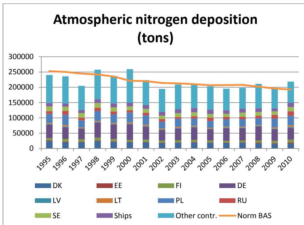
Figure 2.3. Annual actual atmospheric total nitrogen deposition from HELCOM Contracting Parties, Baltic Sea shipping (Ships) and other countries and sources (Other contr.) on the Baltic Seas and annual normalized total nitrogen to the Baltic Sea (line) during 1995-2010 (tonnes nitrogen).
