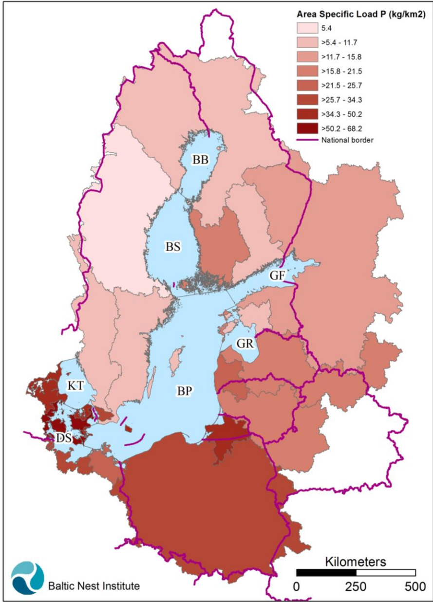
Figure 3.3c. Area-specific riverine phosphorus inputs (kg km -2 ) in 2010 calculated per main sub-catchment and per country. See note to Table 2.2 regarding the pre-conditions on the PLC-5.5 data set.
