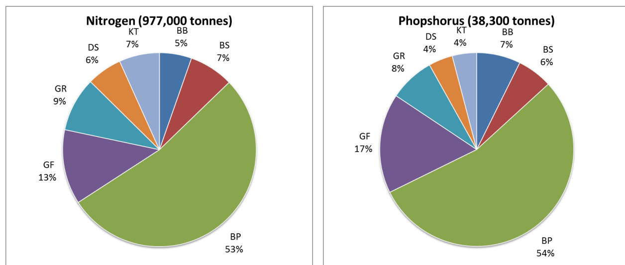
Figures 3.2a and 3.2b. Total actual water- and airborne inputs of nitrogen and phosphorus to the Baltic Sea by sub-basin in 2010. See note to Table 2.2 regarding the preconditions on the PLC-5.5 data set.
