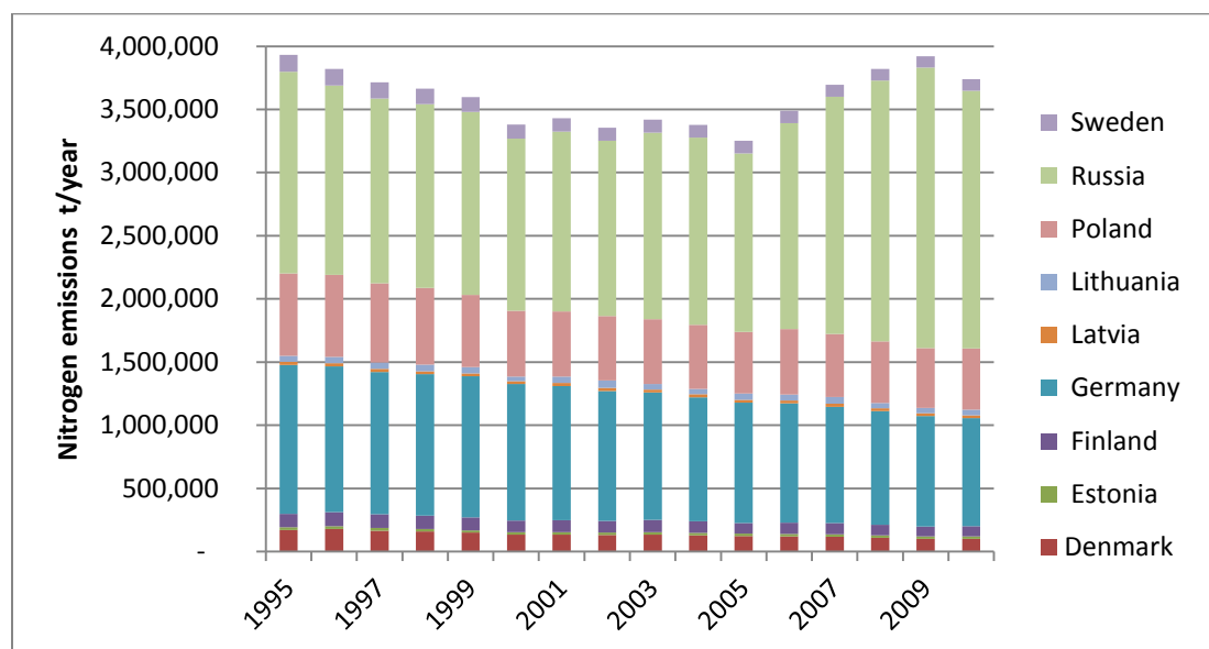
Figure 2.1. Annual atmospheric emissions of total nitrogen from individual HELCOM countries during 1995-2010. Note: the data cover emissions from the entire territories of the countries, except for Russia, where only emissions from the area covered by the EMEP domain are included. This area was significantly extended from 2006 resulting in a large increase of nitrogen emissions from Russia (Source: Bartnicki 2012a).
