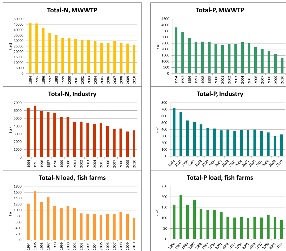
Figure 4.4. Annual direct inputs of total nitrogen and total phosphorus to the Baltic Sea from municipal wastewater treatment plants, MWWTP (top), industrial plants (middle) and fish farms (bottom) discharging directly to the sea during 1994-2010. See note to Table 2.2 regarding the pre-conditions on the PLC-5.5 data set.
