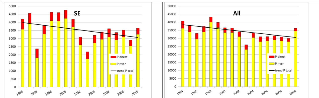
Figure 2.4b. Actual annual total riverine + direct phosphorus inputs by Contracting Party to the Baltic Sea and the total input to the Baltic Sea. The trend line for the flow normalized waterborne total phosphorus input is inserted as a line to indicate possible trend (solid line = a statistically significant trend; dotted line = no statistically significant trend; see further explanations in Chapter 2.4 ). See note to Table 2.2 regarding the pre-conditions on the PLC-5.5 data set.
