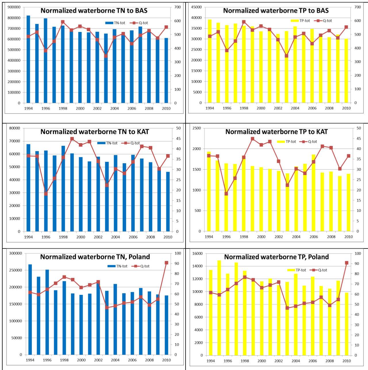
Figure 2.6. Flow normalized annual waterborne (riverine + direct) nitrogen and phosphorus inputs (left-axis) and water flow – Q_{tot} (right y-axis) to the Baltic Sea (top), the Kattegat (middle) and from Poland (bottom). See note to Table 2.2 regarding the pre-conditions on the PLC-5.5 data set.
