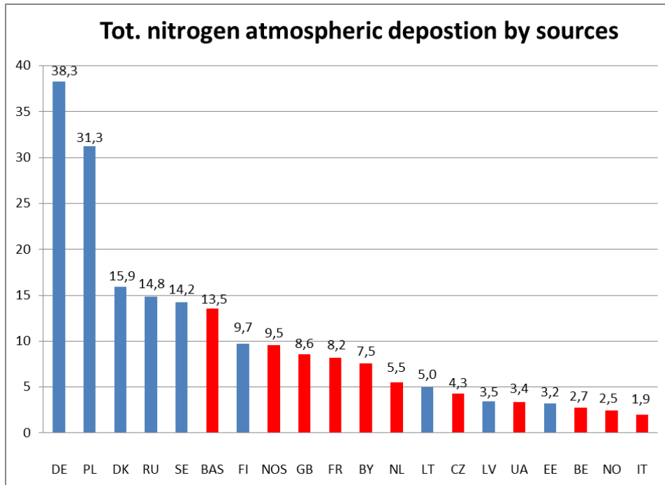
Figure 4.3. Top twenty biggest contributors of atmospheric total nitrogen deposition (kilo tonnes nitrogen, i.e. DE= 38,300 tonnes nitrogen) to the Baltic Sea in 2010. Non-HELCOM countries or sources outside HELCOM area are in red. BAS = Baltic Sea shipping; BE = Belgium; BY = Belarus; NOS = North Sea shipping; UA = Ukraine.
