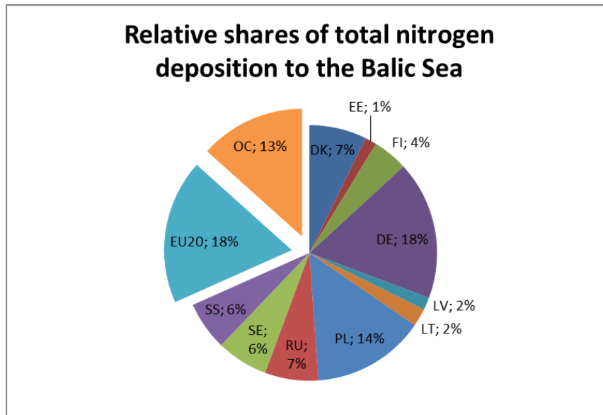
Figure 4.2. The relative share of different sources of actual atmospheric total nitrogen deposition to the Baltic Sea in 2010.
