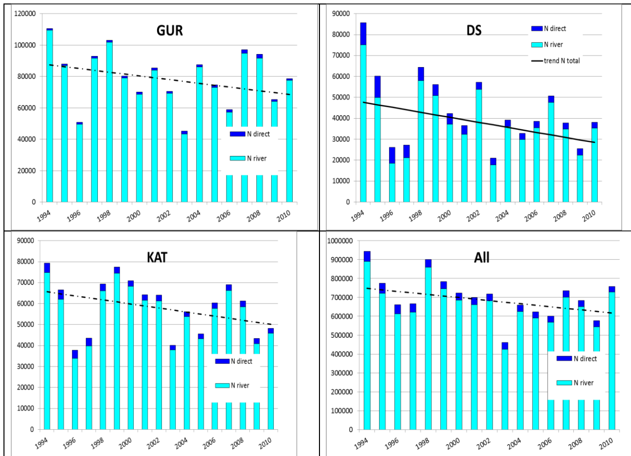
Figure 2.5a. Actual annual total riverine + direct nitrogen inputs to Baltic Sea sub-basin and total to the Baltic Sea. The trend line for the flow normalized waterborne total nitrogen input is inserted as a line to indicate possible trend (solid line = a statistically significant trend; dotted line = no statistically significant trend; see further explanations in Chapter 2.4 ). See note to Table 2.2 regarding the pre-conditions on the PLC-5.5 data set.
