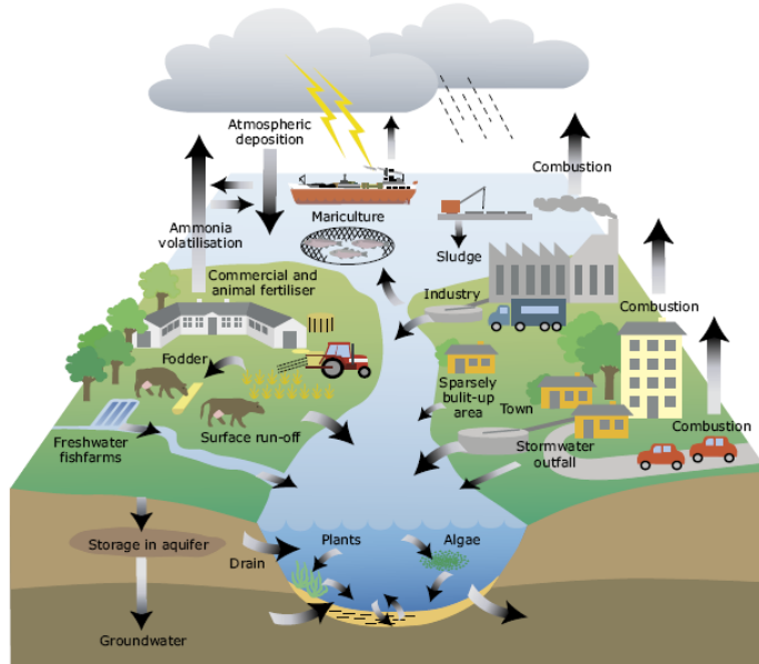
Figure 1.2. Different sources of nutrients to the sea and examples of nitrogen and phosphorus cycles. The flow related to ammonia volatilization shown in the figure applies only to nitrogen. In this report, also combustion and atmospheric deposition deal only with nitrogen. Emissions of phosphorus to the atmosphere by dust from soils are not shown in the figure. (Source: Ærtebjerg et al. 2003).
