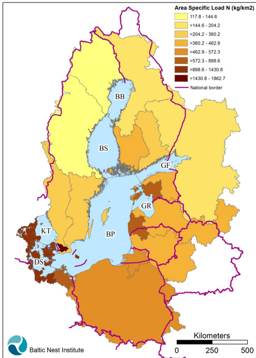
Figure 3.3b. Area-specific riverine nitrogen inputs ( \text{kg km}^{-2} ) in 2010 calculated per main sub-catchment and per country. See note to Table 2.2 regarding the pre-conditions on the PLC-5.5 data set.
