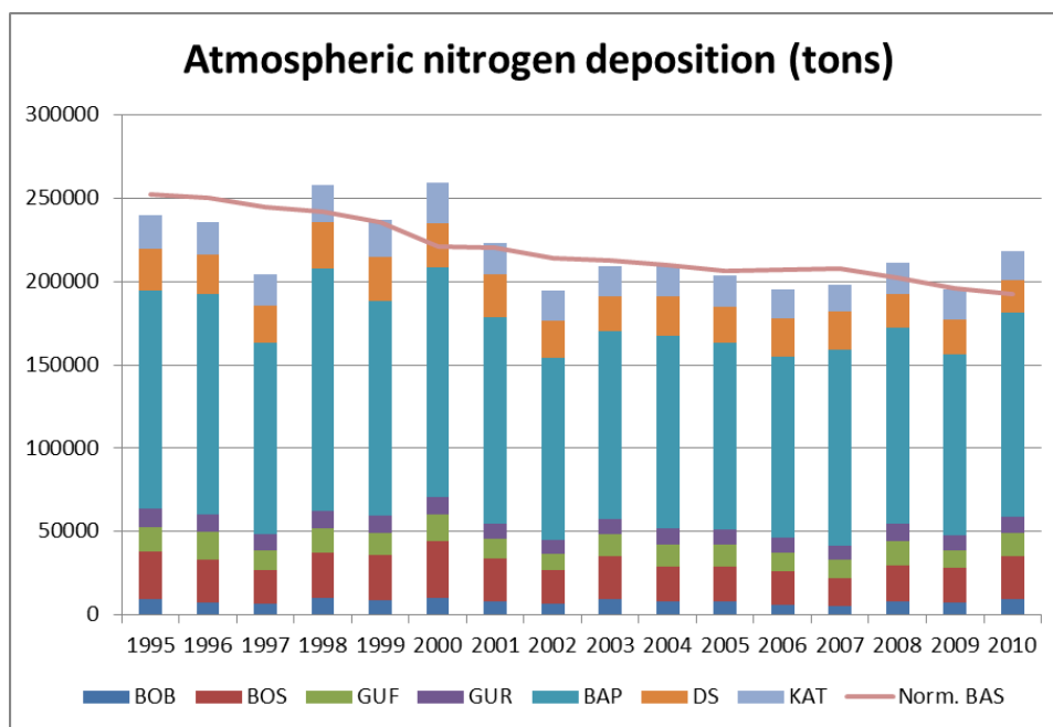
Figure 2.2. Annual actual atmospheric total nitrogen deposition (not normalized) on the Baltic Sea main sub-basins and annual normalized total nitrogen to the Baltic Sea (line) during 1995-2010 (tonnes nitrogen).
