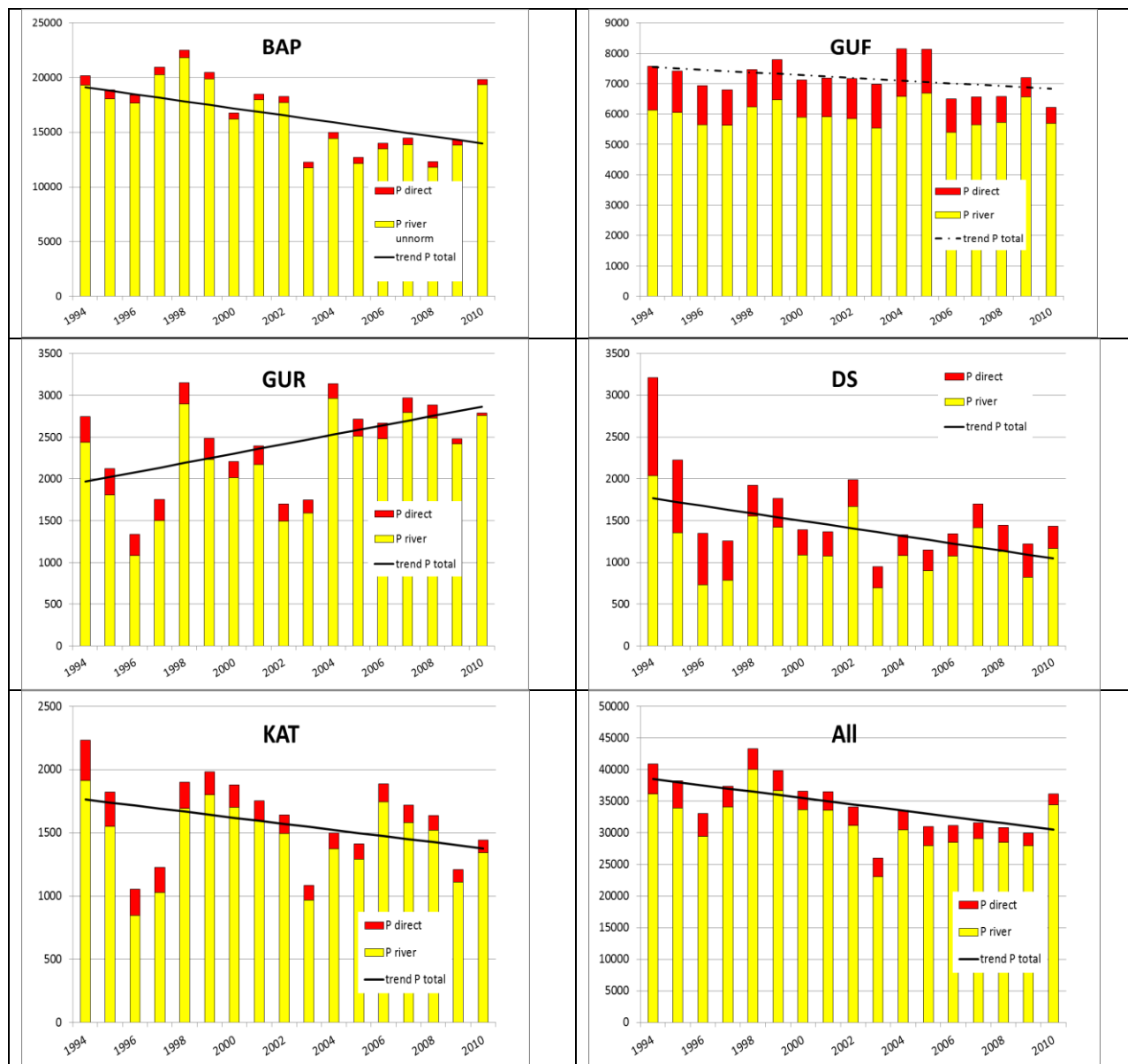
Figure 2.5b. Actual annual total riverine + direct phosphorus inputs to Baltic Sea sub-basin and the total input to the Baltic Sea. The trend line for the flow normalized waterborne total phosphorus input is inserted to indicate possible trend (solid line = a statistically significant trend; dotted line = no statistically significant trend; see further explanations in Chapter 2.4 ). See note to Table 2.2 regarding the pre-conditions on the PLC-5.5 data set.
