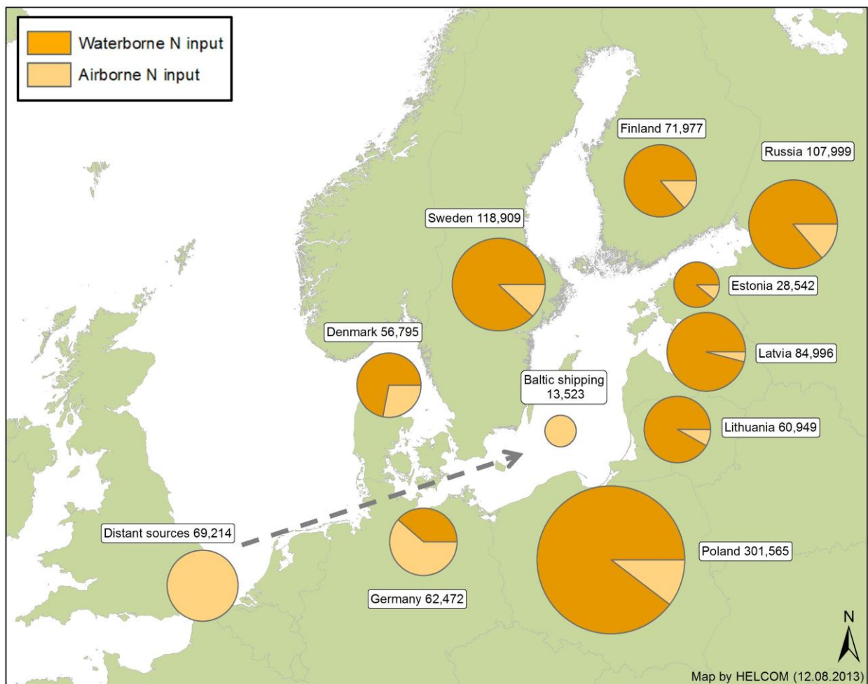
Figure 4.1. Total actual inputs of water- and airborne nitrogen from HELCOM countries, Baltic Sea shipping and distant sources to the Baltic Sea in 2010. See note to Table 2.2 regarding the pre-conditions on the PLC-5.5 data set.
